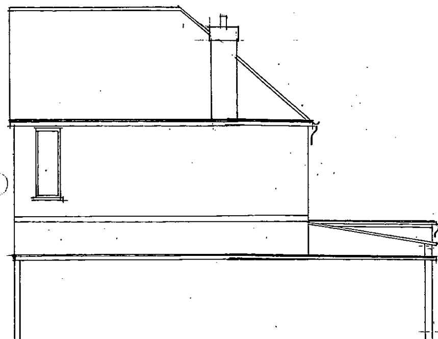
SOUTH ELEVATION.
