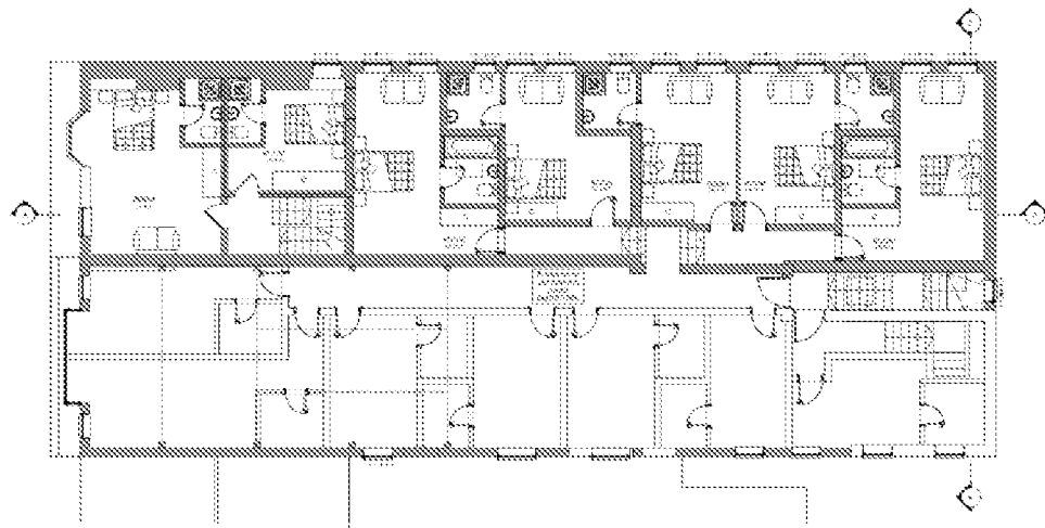
FIRST FLOOR 1:100 @ A2
