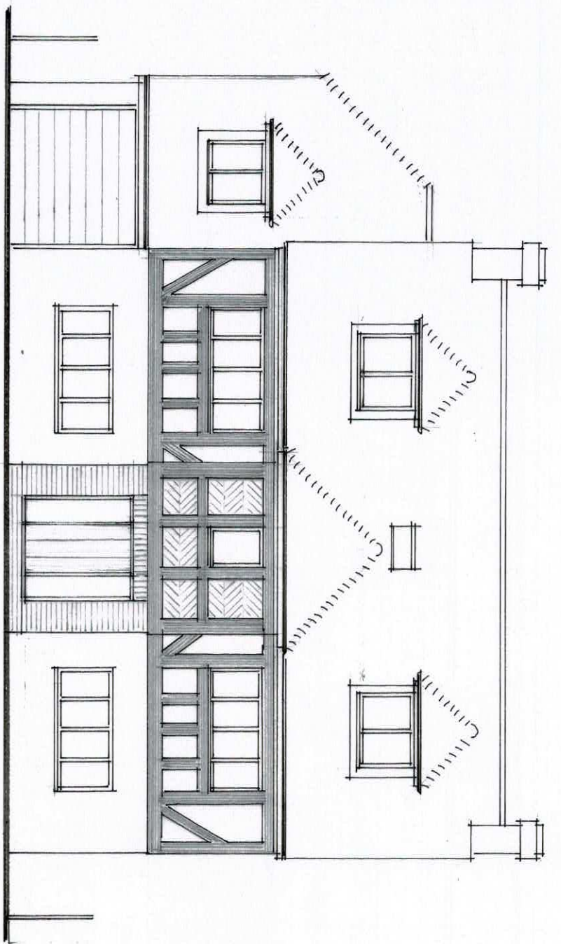
FRONT ELEVATION (SE) PROPOSED 1-100
