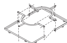
Removable central supports - square
