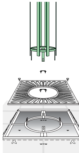
Tree protection system showing tree guard fitted with bolt and frame fixings.
