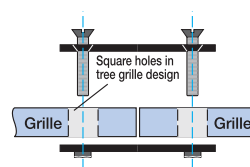
CLAMP TYPE A (Square hole design)
