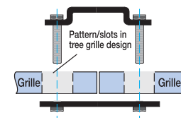
CLAMP TYPE B (all other designs)
