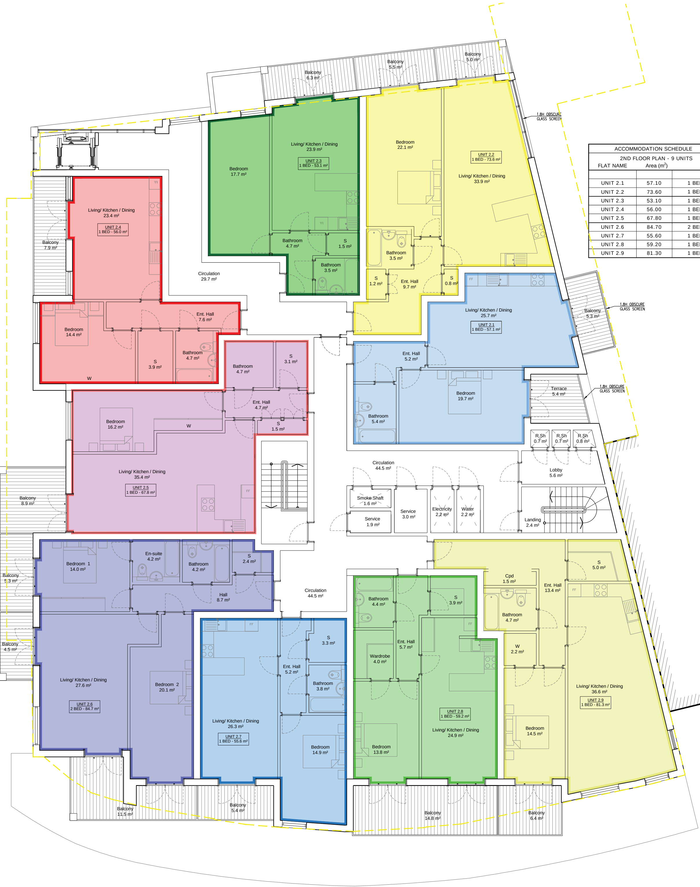
2ND FLOOR PLAN Sc. 1:100
