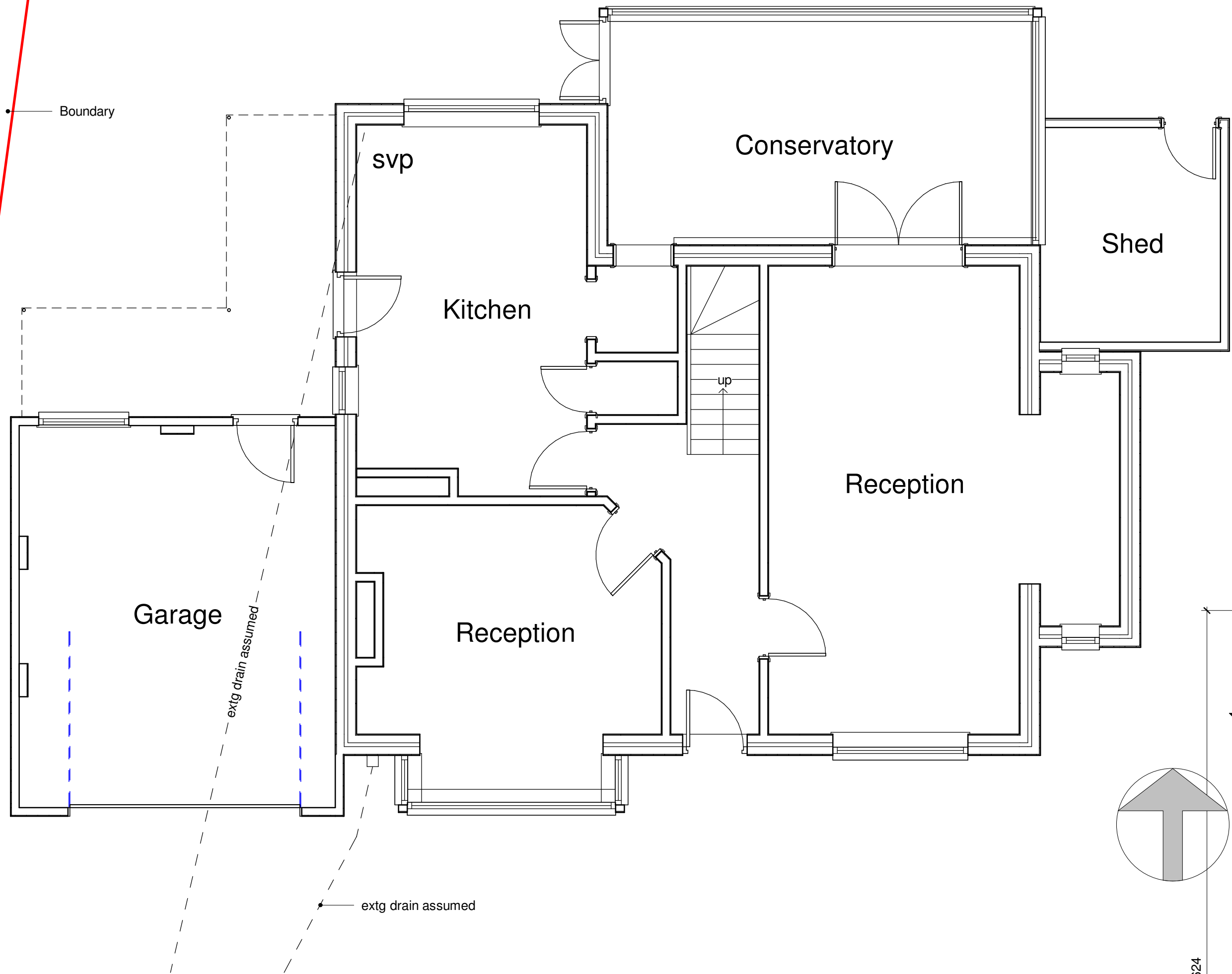
1 FFL Ground Existing 1 : 50
