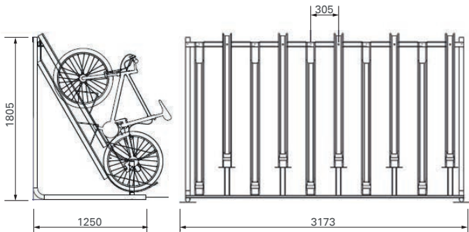
FalcoVert-Plus, part code 00.555.xxxUK
