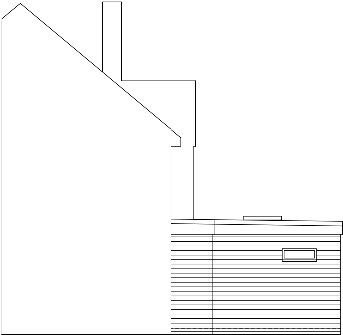
PART SIDE ELEVATION (NORTH) SHOWING PROPOSED EXTENSION
