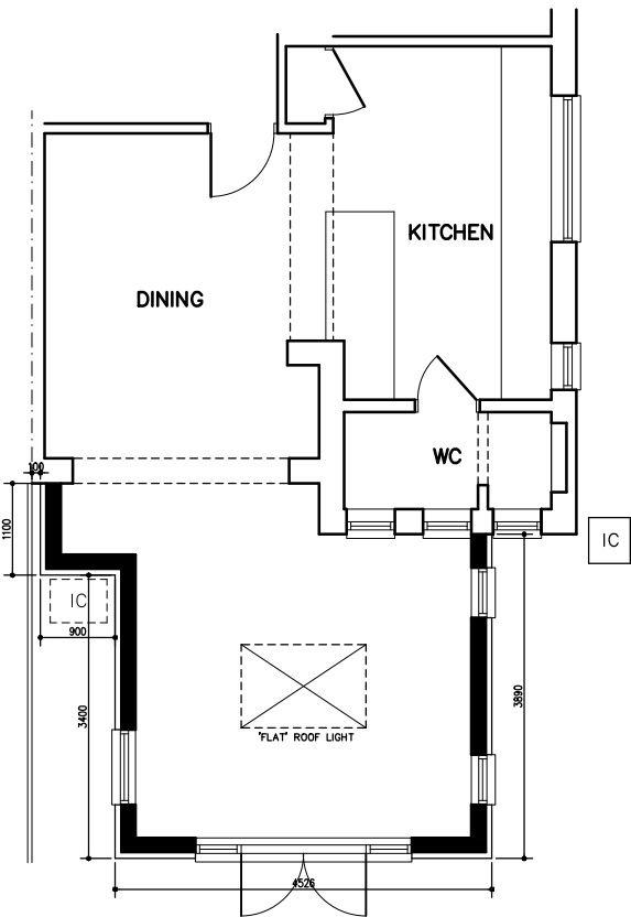
PART GROUND FLOOR PLAN SHOWING PROPOSED EXTENSION
