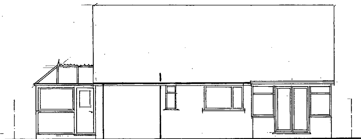
WEST ELEVATION.
