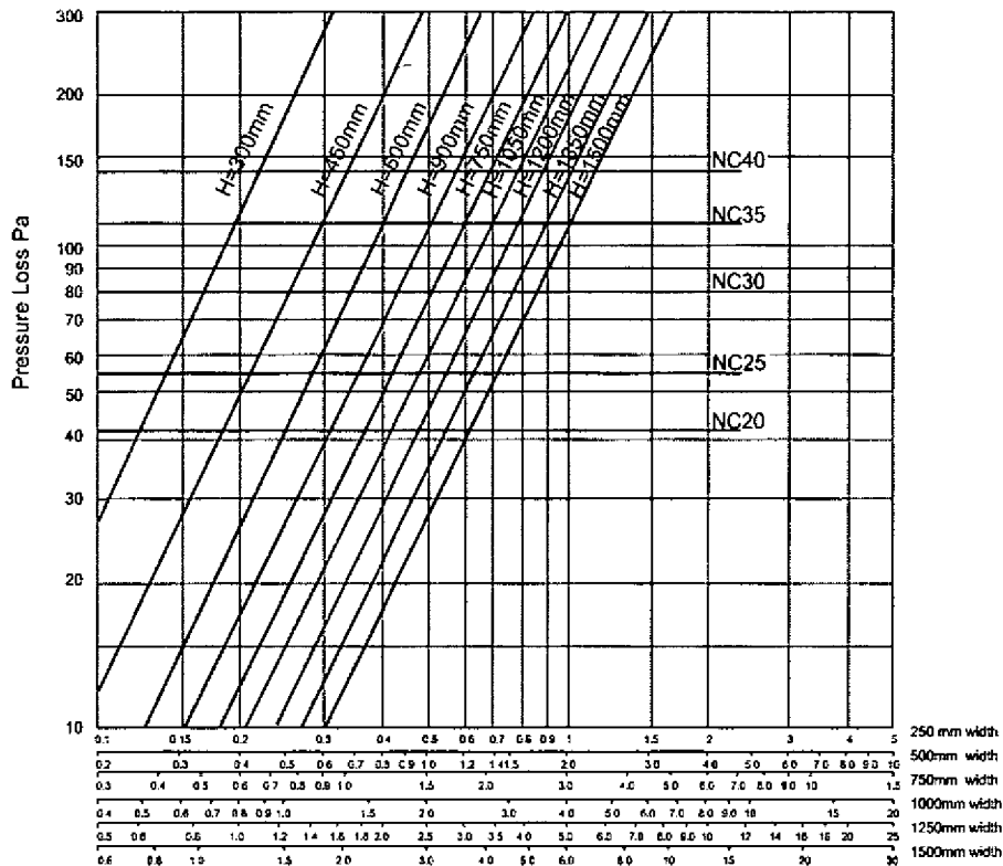
Chart 2 - Resistance to Air Flow Type WS/75
