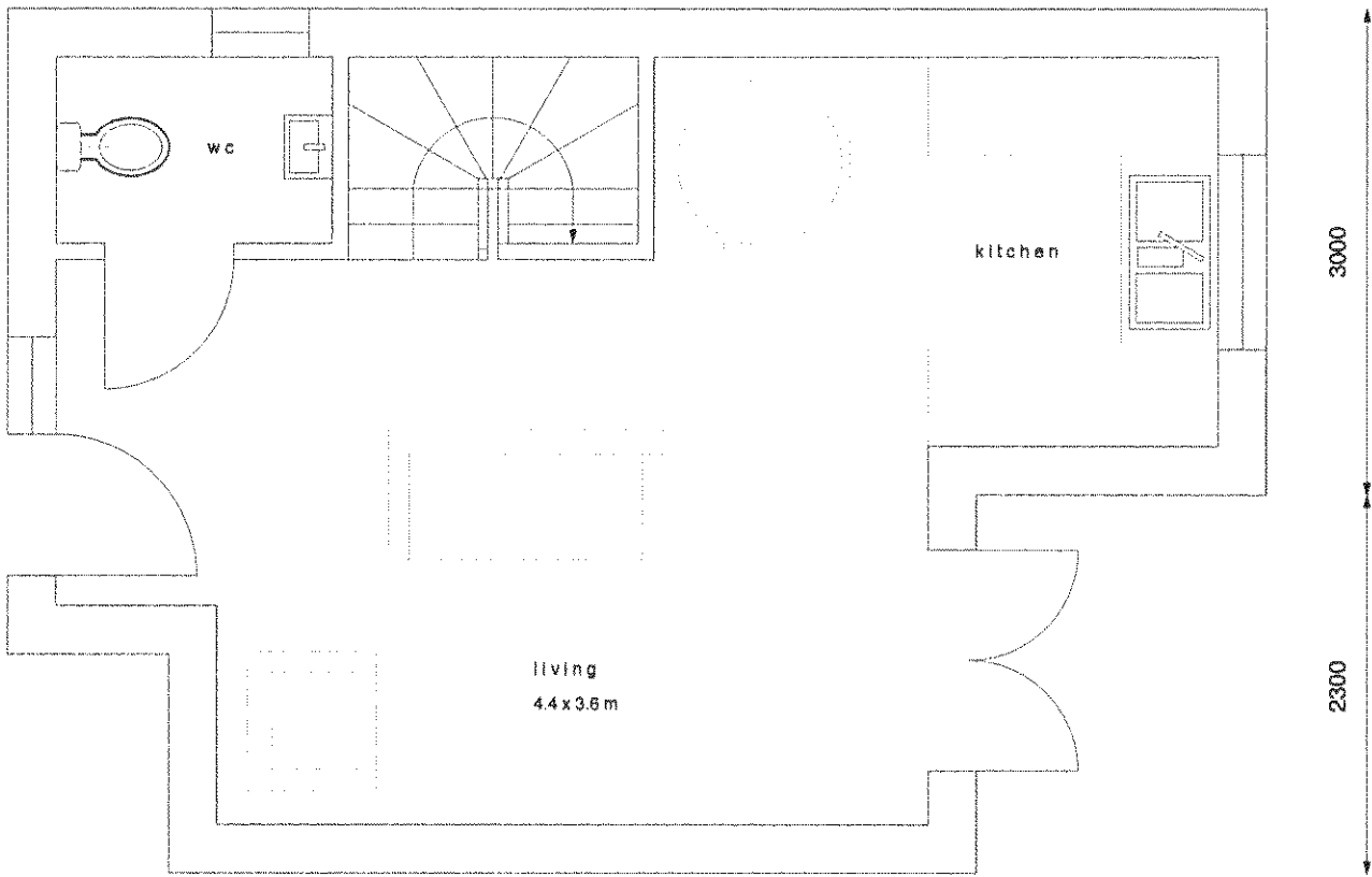
Proposed Ground Floor Plan at 1:50 scale
