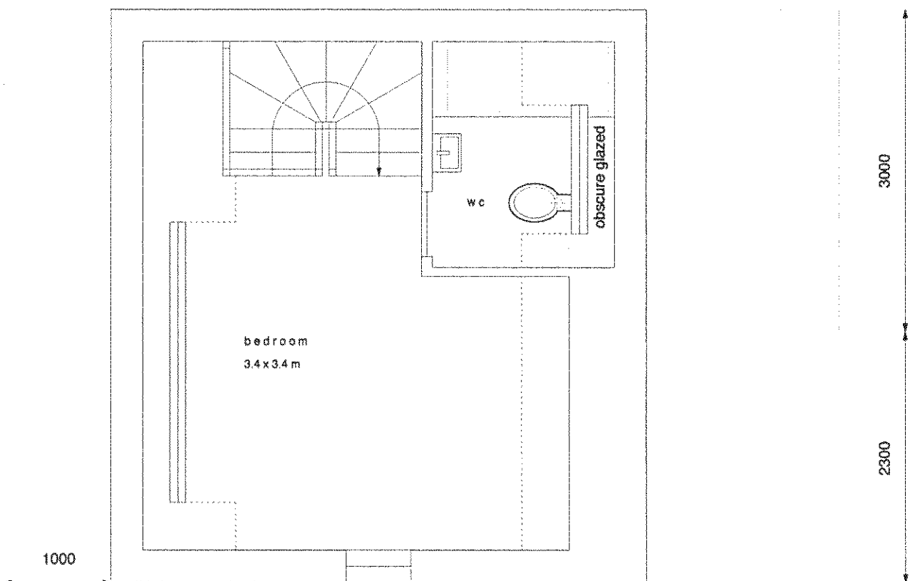
Proposed First Floor Plan at 1:50 scale
