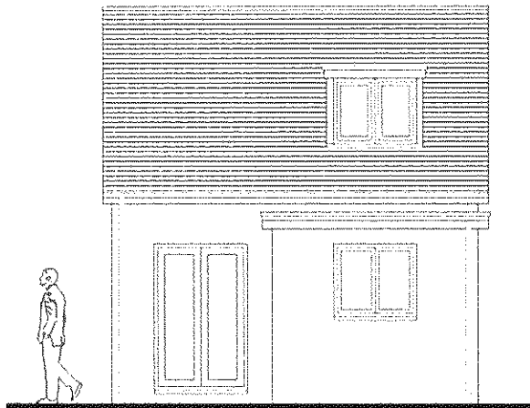
Proposed North West Elevation at 1:100 scale
