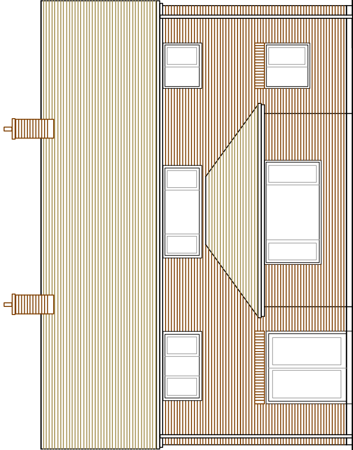
EXISTING SOUTH ELEVATION 1:100
