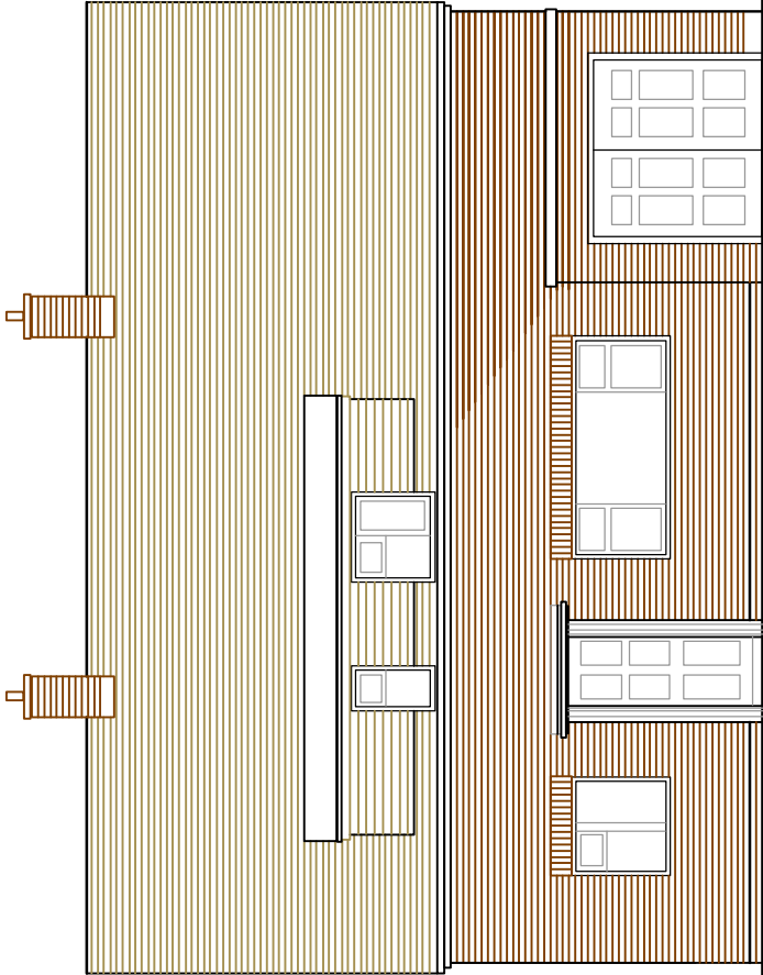
EXISTING NORTH ELEVATION 1:100
