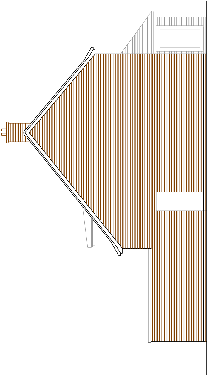
EXISTING WEST ELEVATION 1:100
