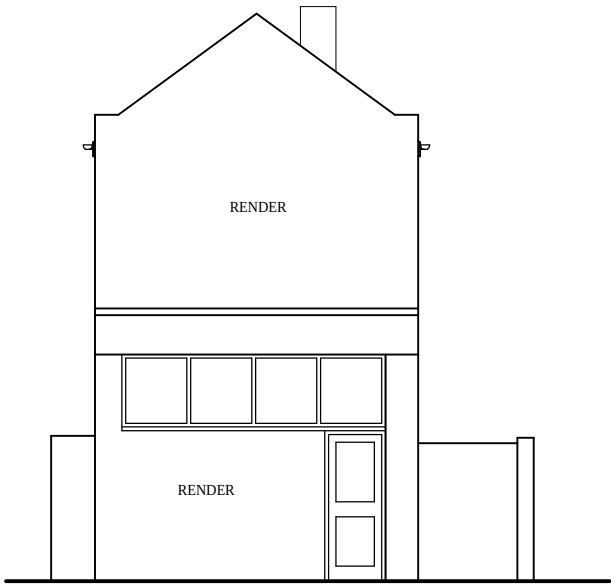
NORTH WEST ELEVATION (FRONT)
