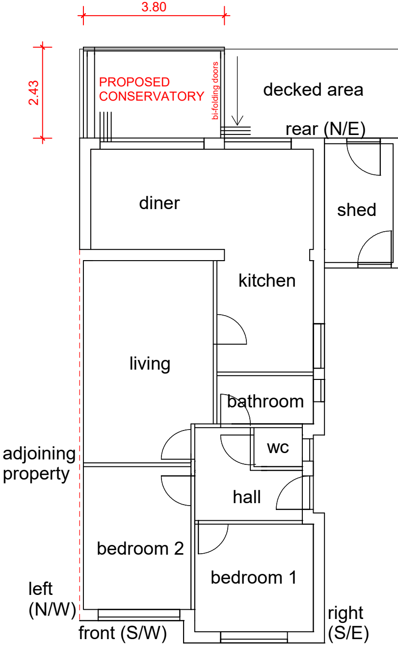
GROUND FLOOR LAYOUT
