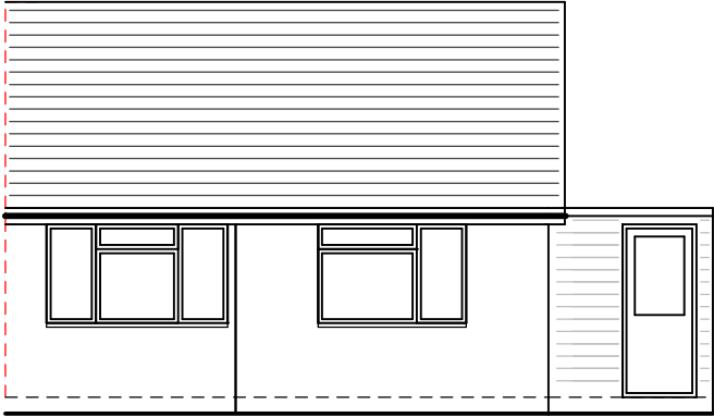
front (south west) elevation
