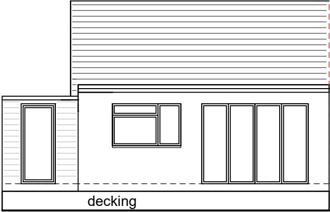
rear (north east) elevation
