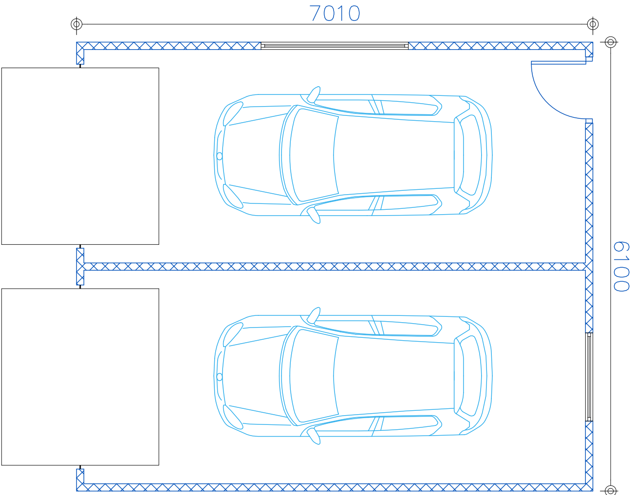
PROPOSED FLOOR PLAN scale 1_50
