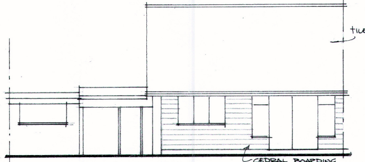
REAR ELEVATION SOUTH
