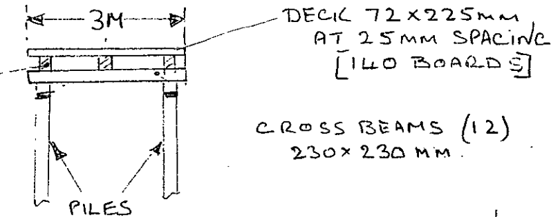
CROSS SECTION
