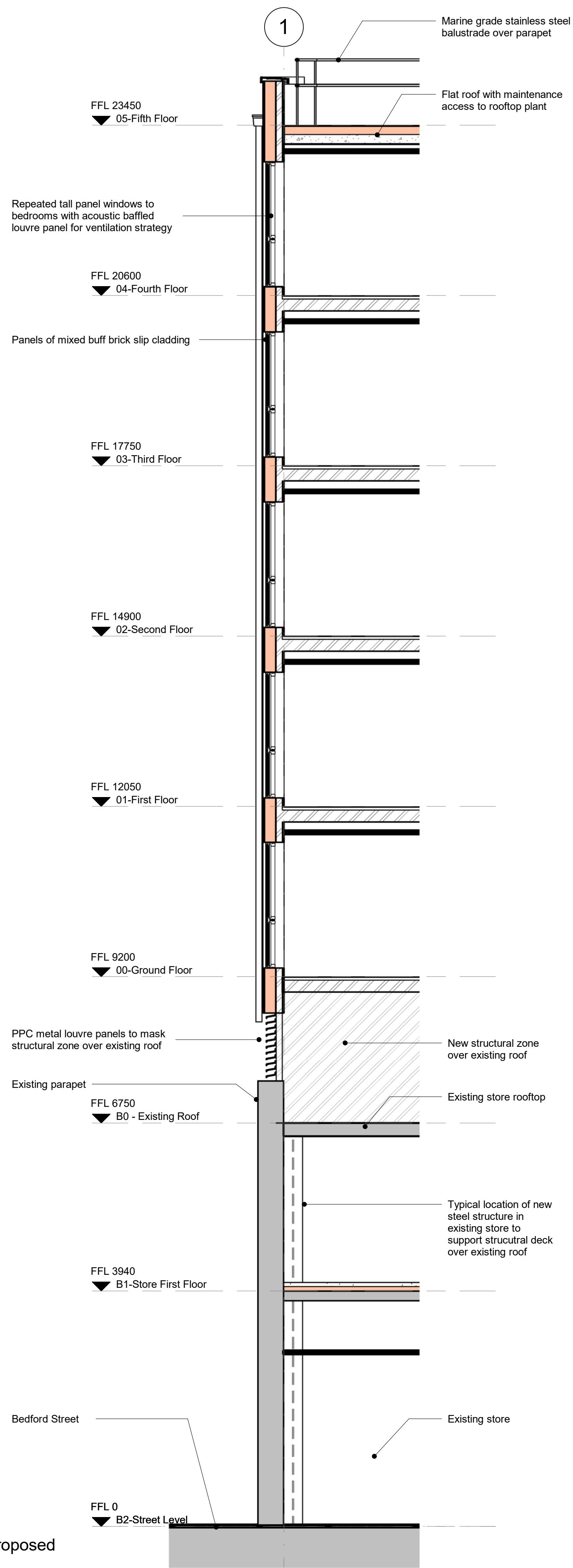
Bay Elevation Proposed 1:50
