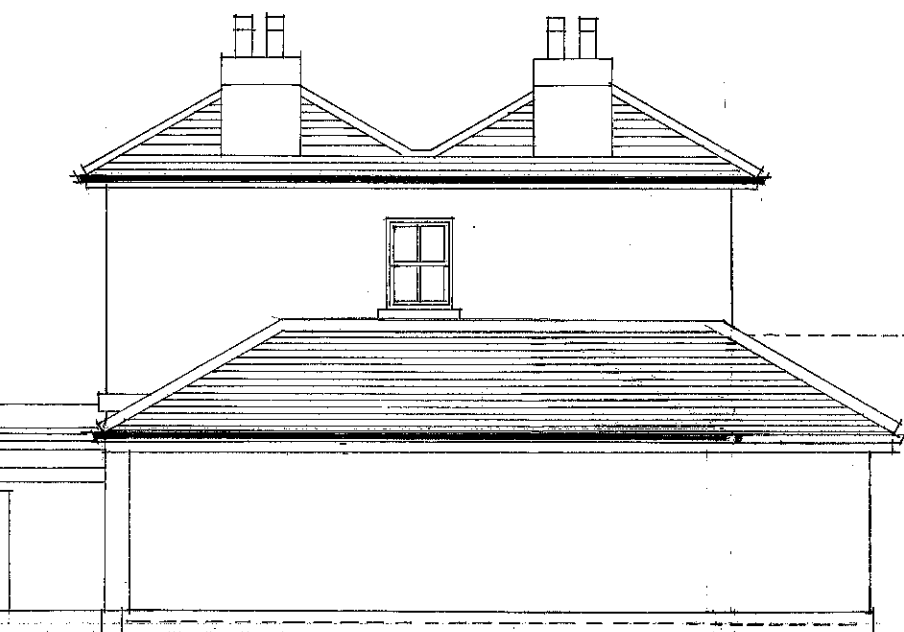
EAST ELEVATION TO 12 CHICHESTER ROAD
