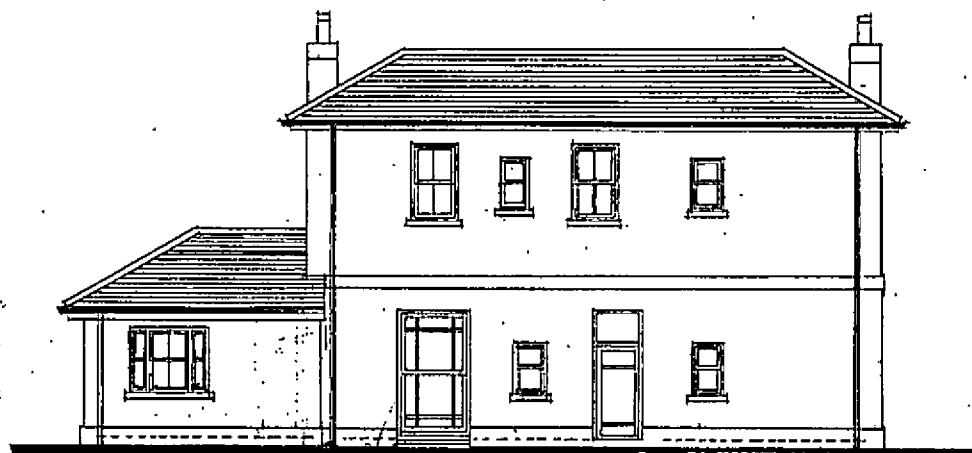
NORTH ELEVATION OF MANOR HOUSE Original openings restored
