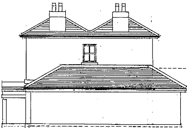
EAST ELEVATION TO 12 CHICHESTER ROAD
