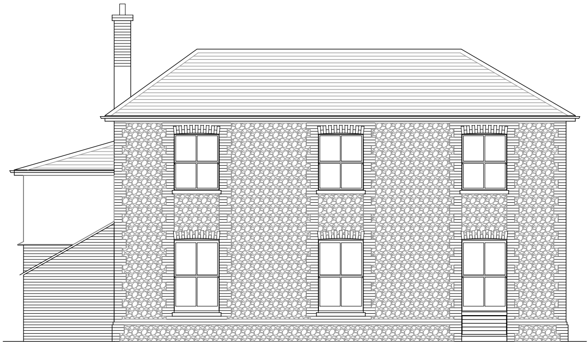
South Elevation
