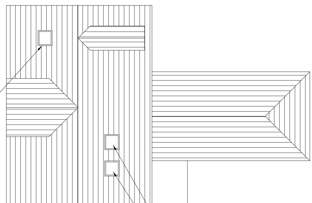
+03 Roof Plan 1:100
