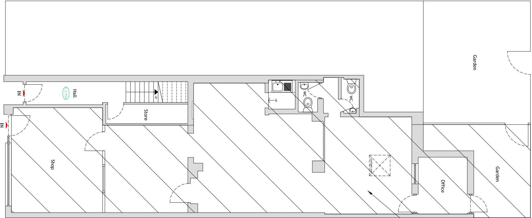
+00 Ground Floor Plan 1:100
