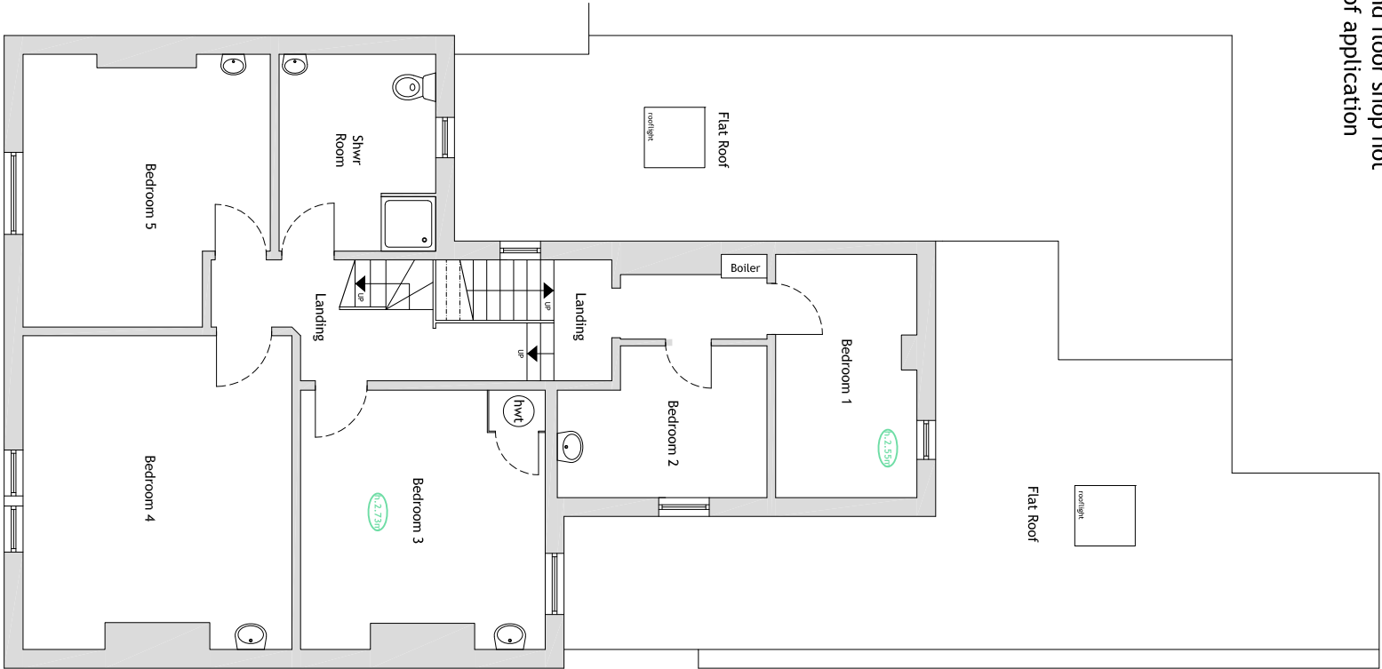
+01 First Floor Plan 1:100
