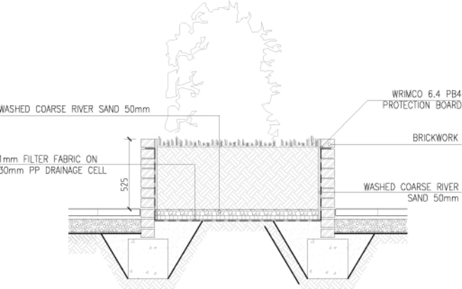
SECTION A-A: PLANTER SECTION, Sc. 1:20
