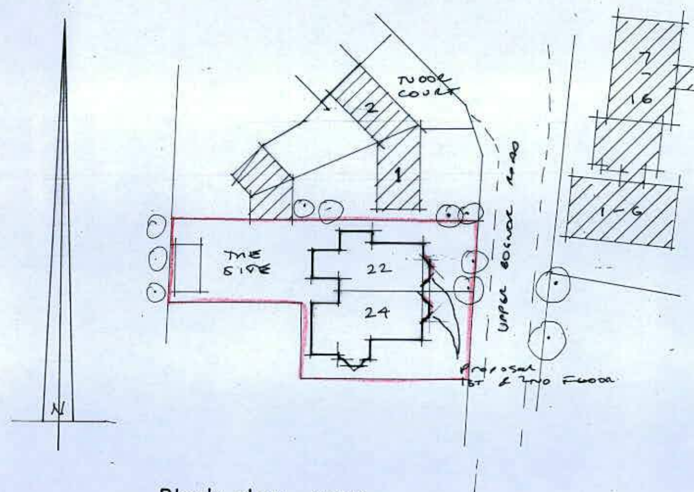
Block plan 1:500
