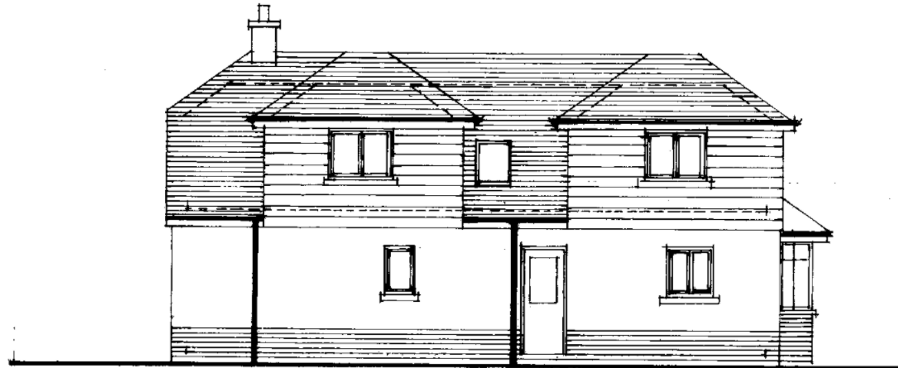
EAST ELEVATION
