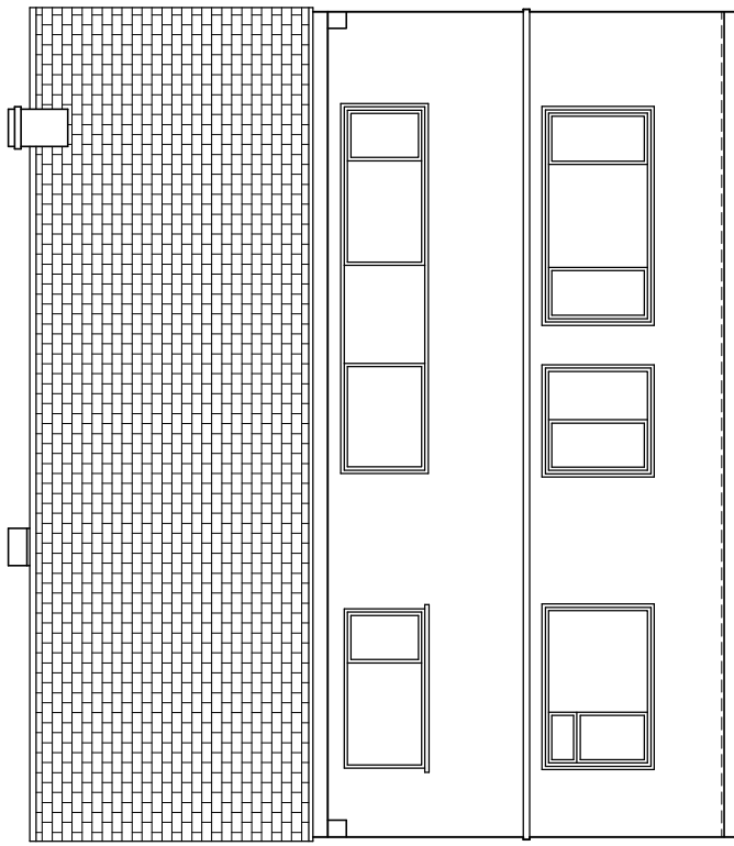
REAR (SOUTH-EAST)
