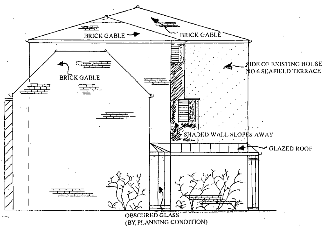
WEST (PROPOSED)
