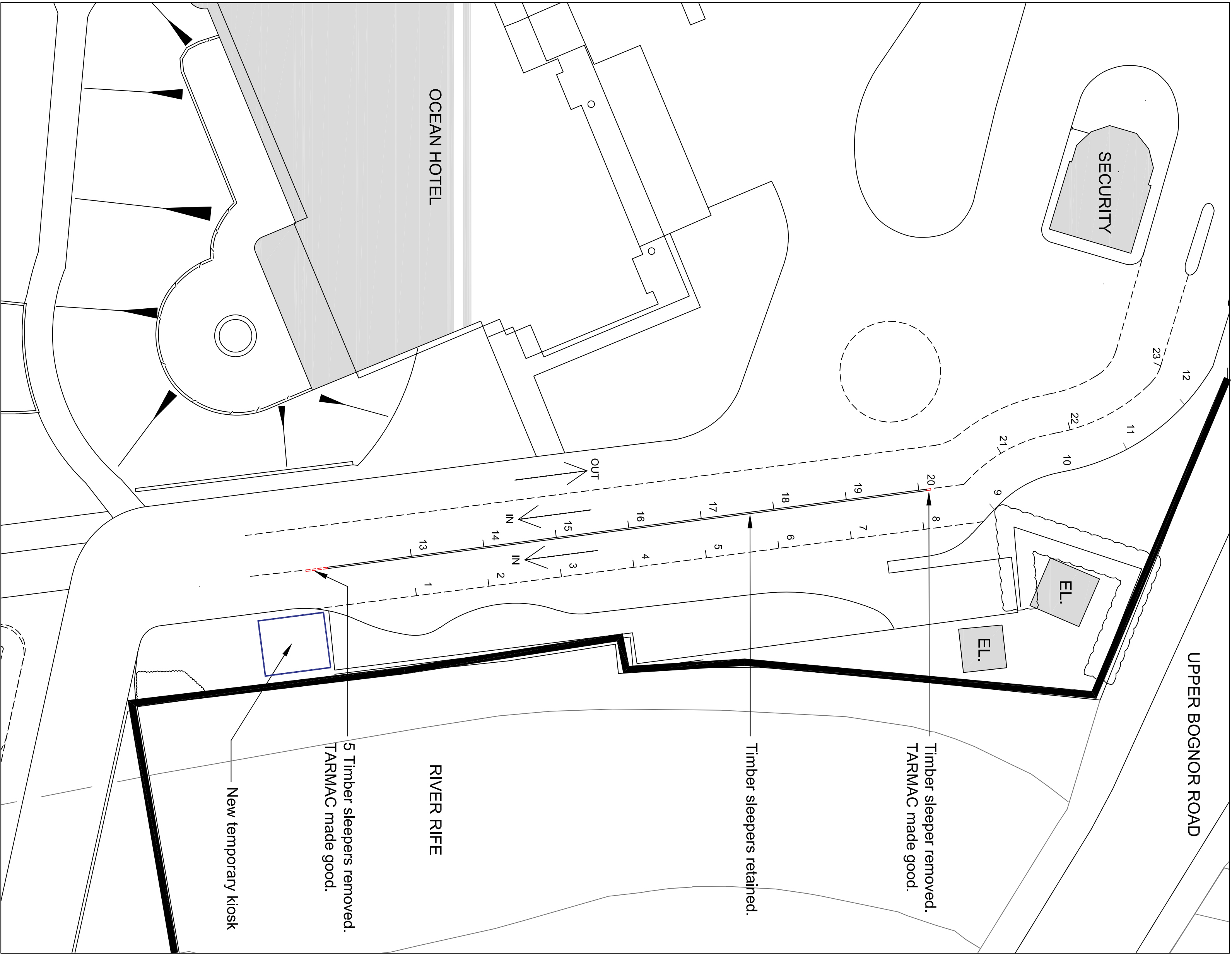
PROPOSED ENTRANCE KIOSK
