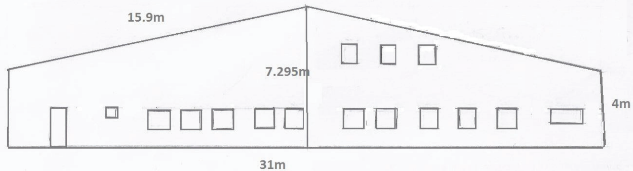
EXISTING WEST ELEVATION
