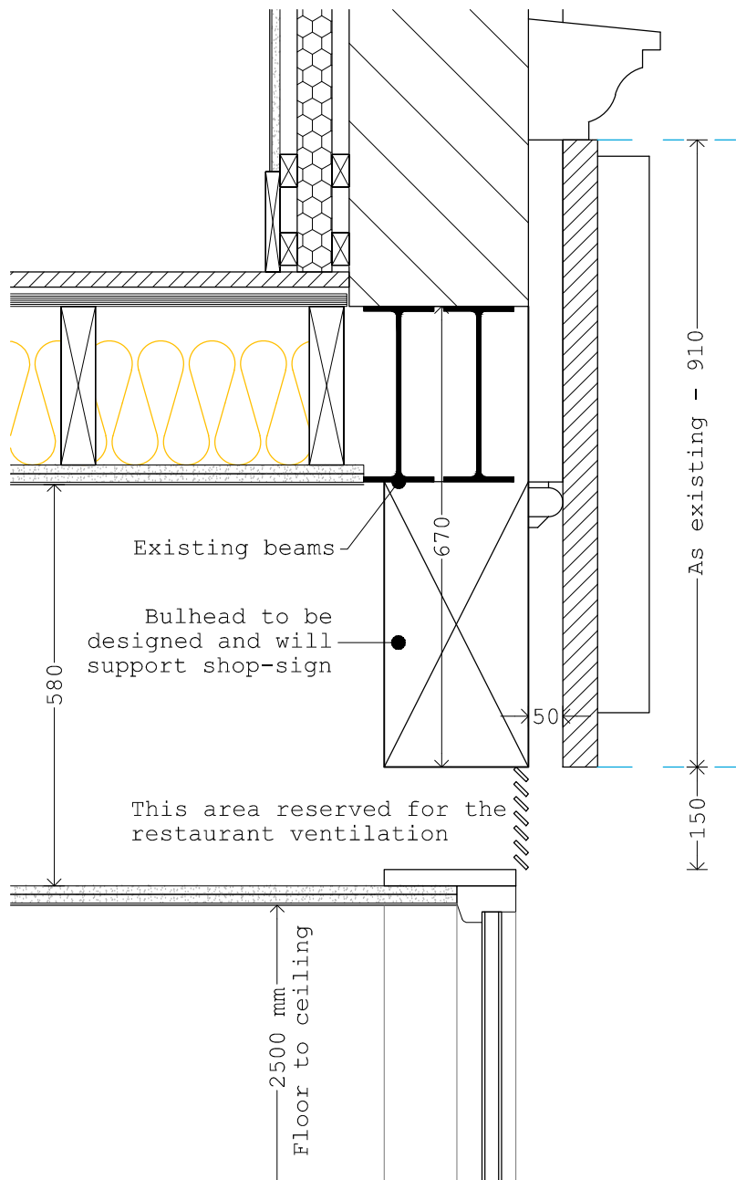
Section - Scale 1:10
