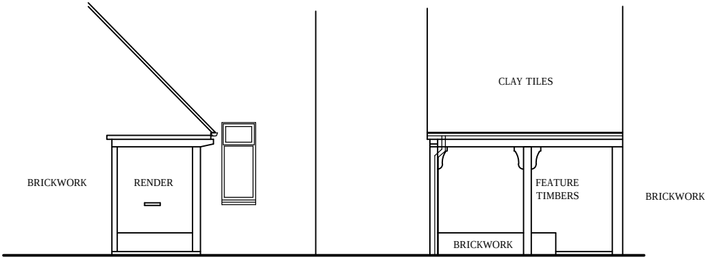
NE ELEVATION 15 STURGES ROAD ENTRANCE
