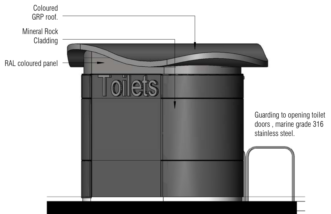
West Elevation 1 : 50
