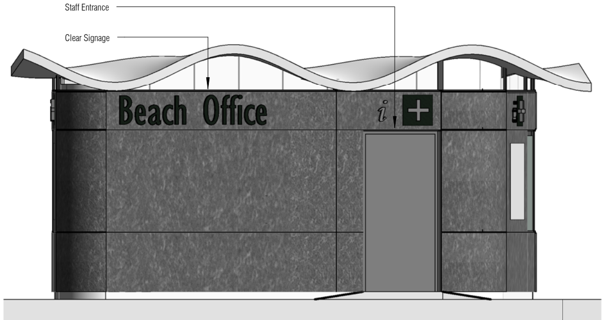
Beach Office North Elevation 1 : 50
