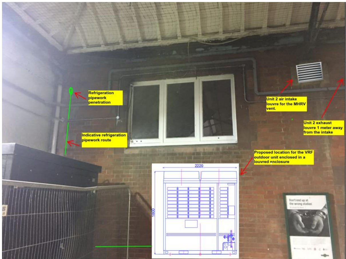
Figure 1 : Outdoor VRF unit proposed location 1
