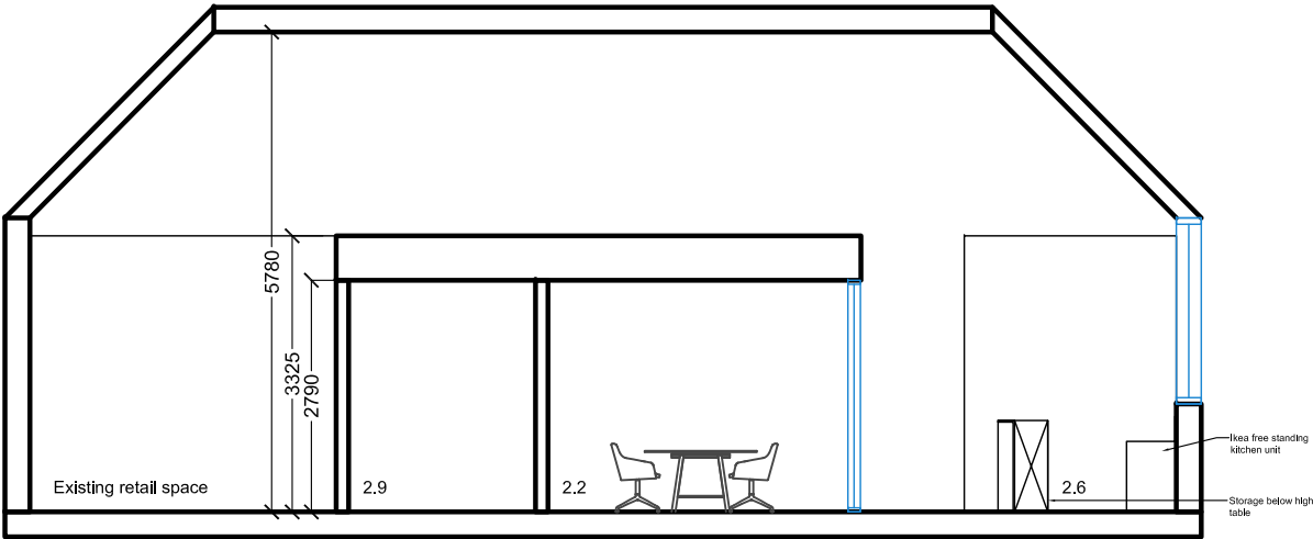
SECTION DD Proposed
