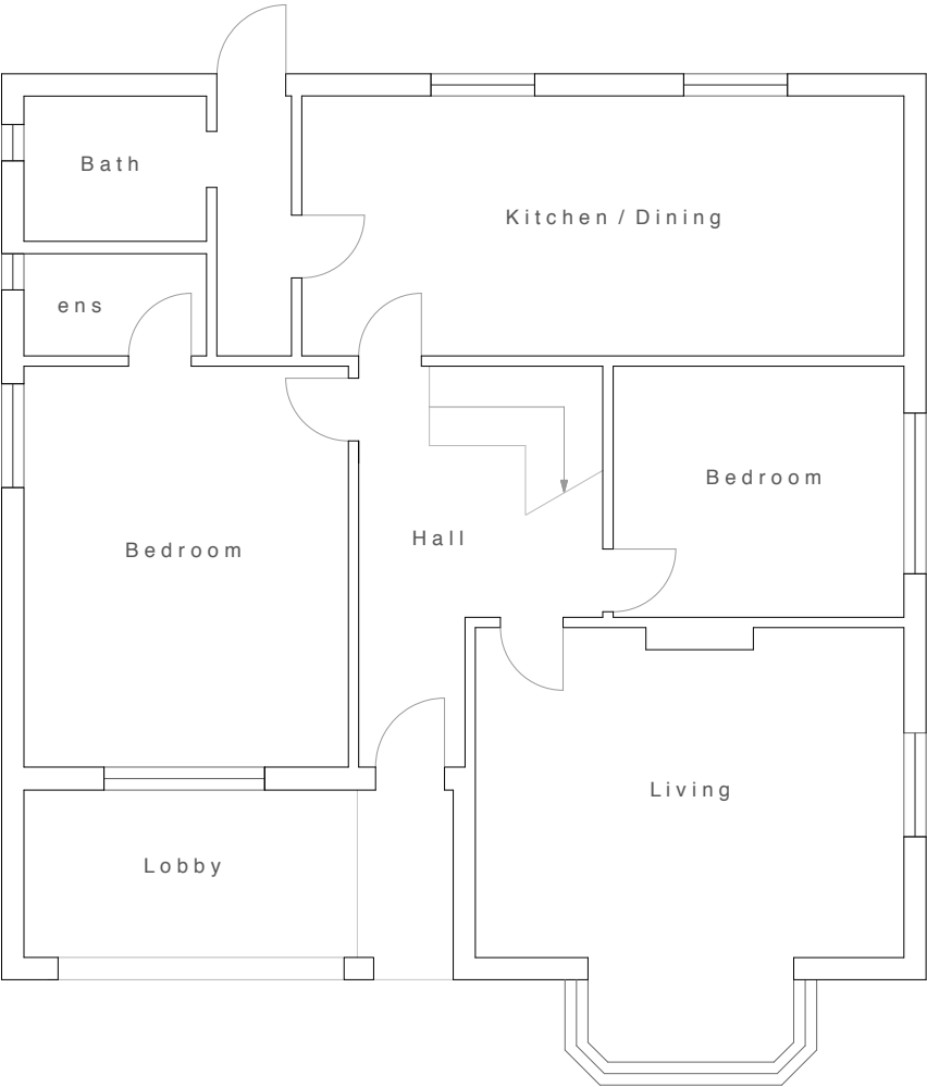
Existing Ground Floor Plan at 1:100 scale
