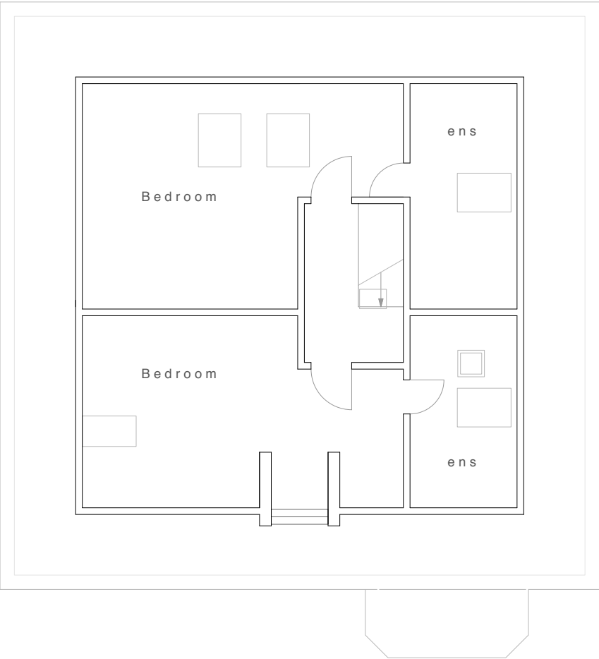
Existing First Floor Plan at 1:100 scale
