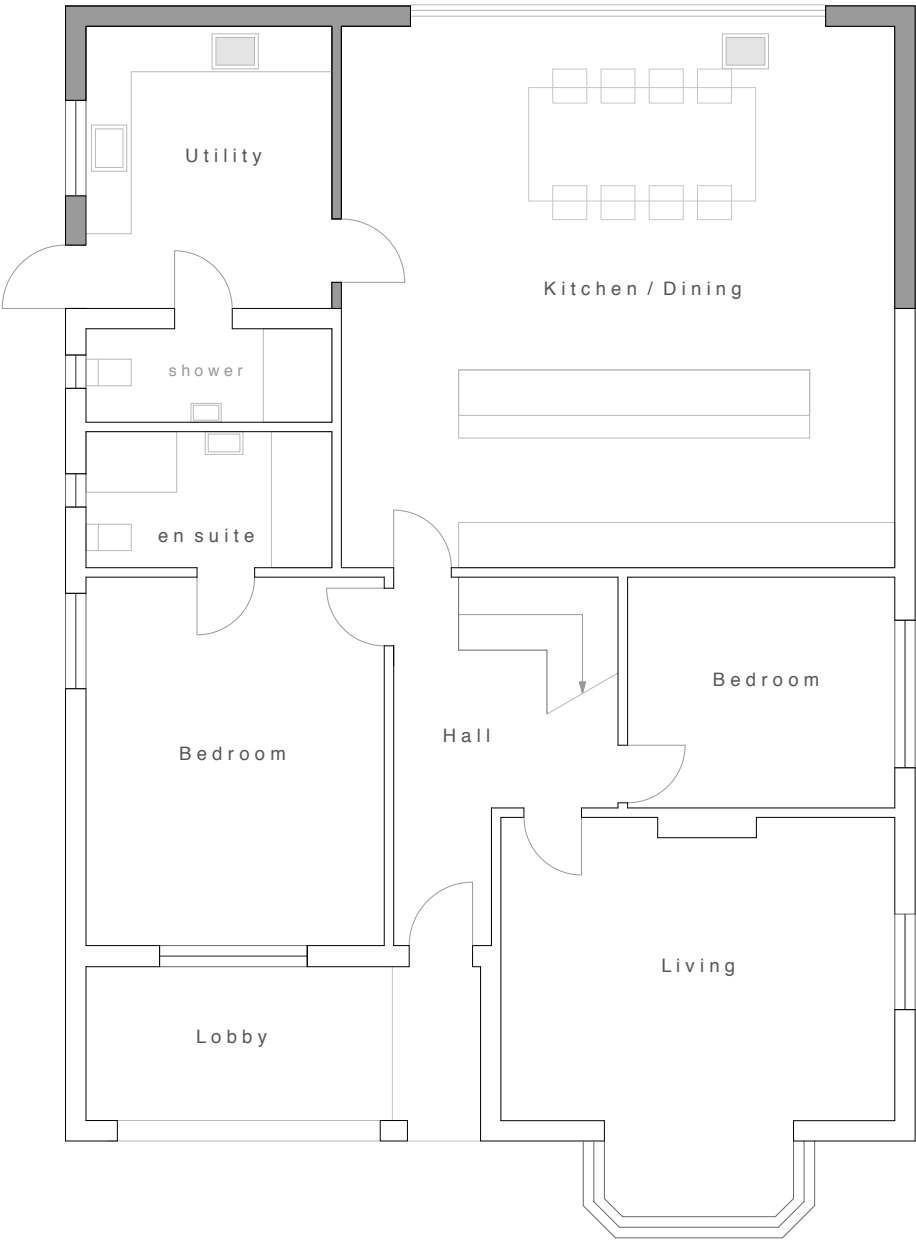
Proposed Ground Floor Plan at 1:100 scale
