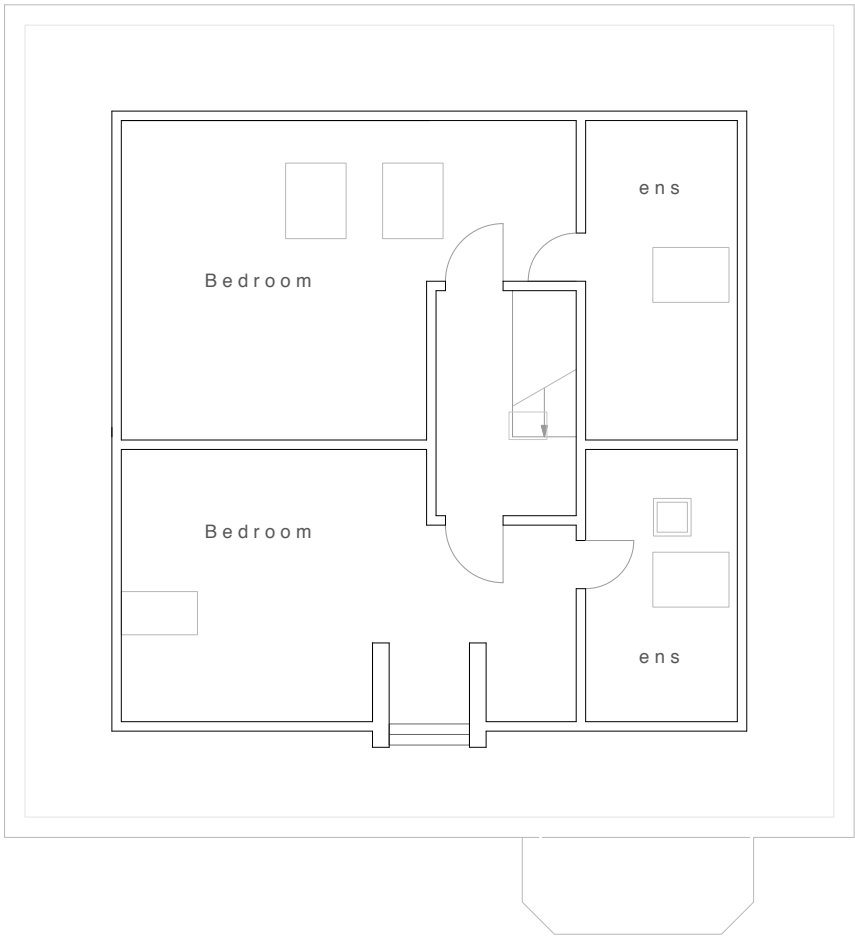
Existing First Floor Plan at 1:100 scale REFERENCE
