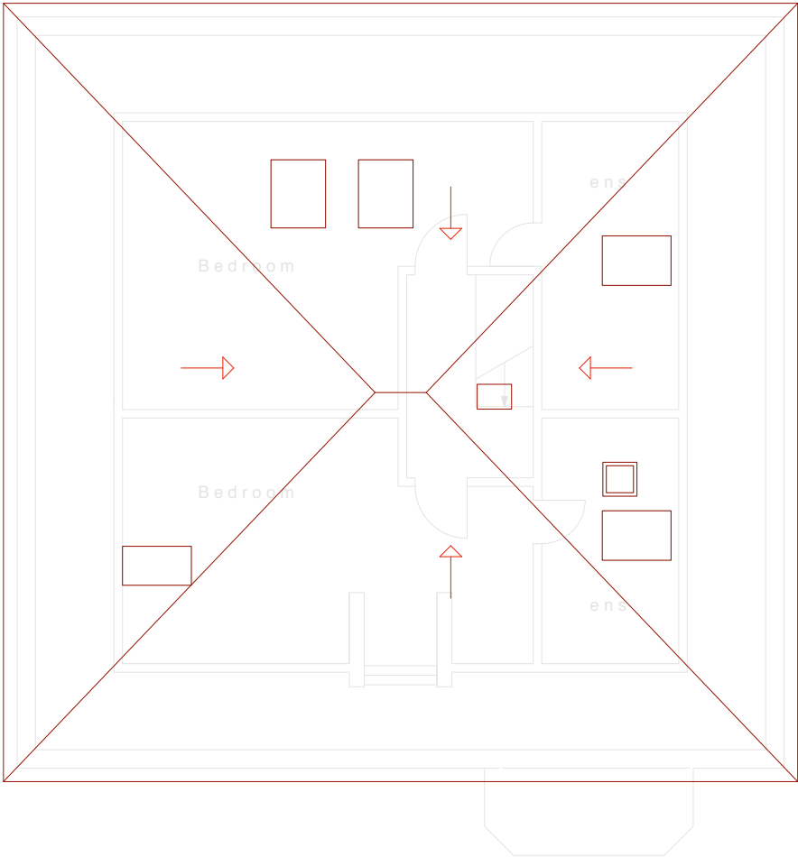
Existing Roof Plan at 1:100 scale
