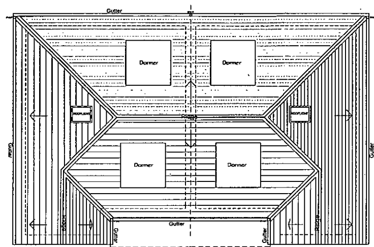
Roof plan
