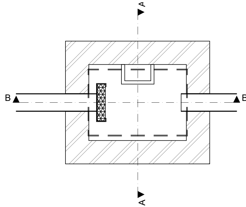
PLAN BRICK CONSTRUCTED CATCHPIT INSPECTION CHAMBER INCORPORATING FLOW CONTROL AND DEBRIS DEVICE SCALE 1: 20
