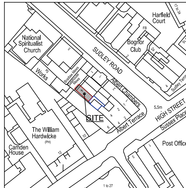
LOCATION PLAN SC. 1:1250
