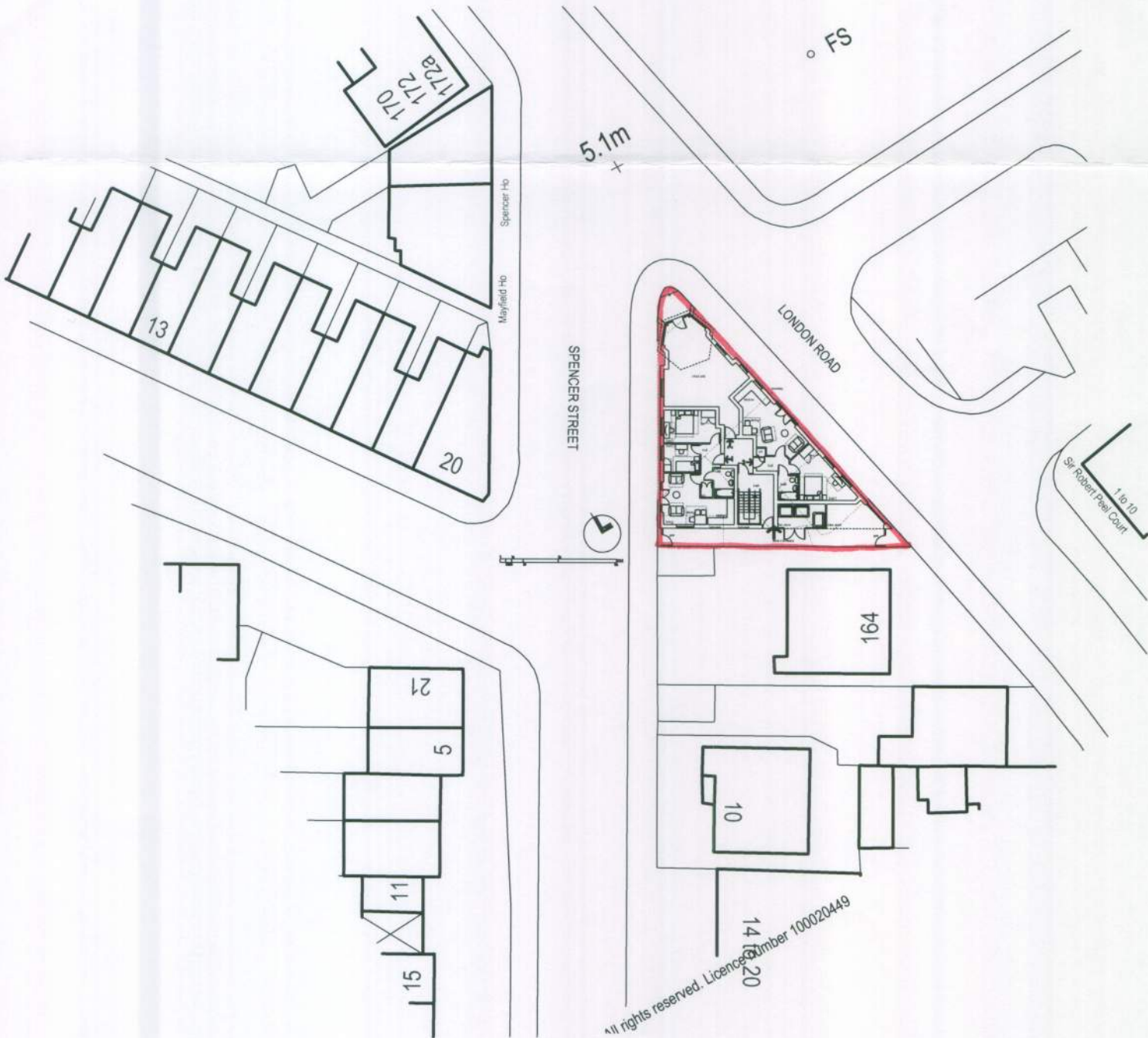
block plan 1:500
