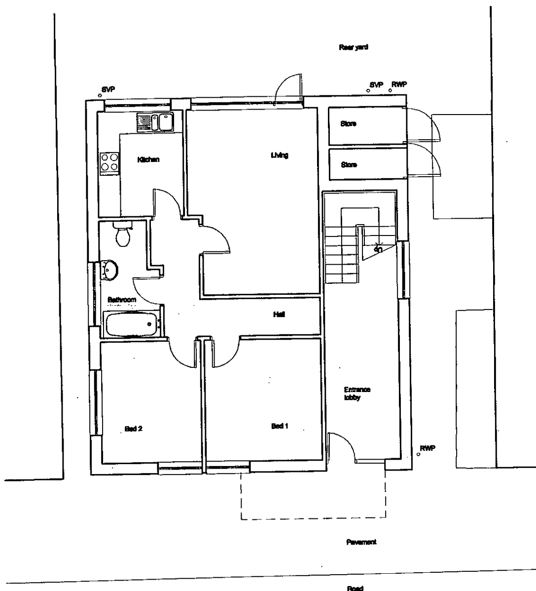
Existing ground floor plan (Flat 1)
