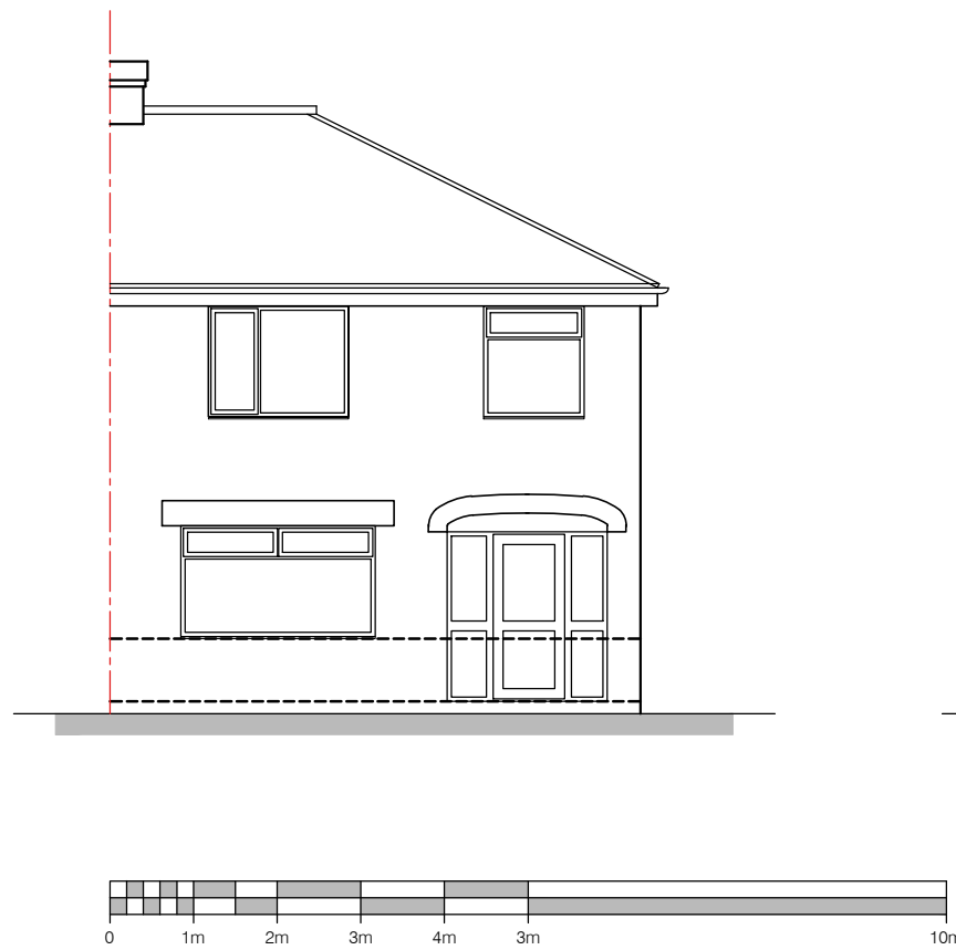
EXISTING North West Elevation
