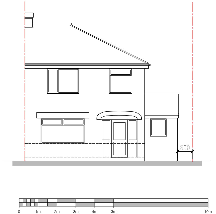
PROPOSED North West Elevation
