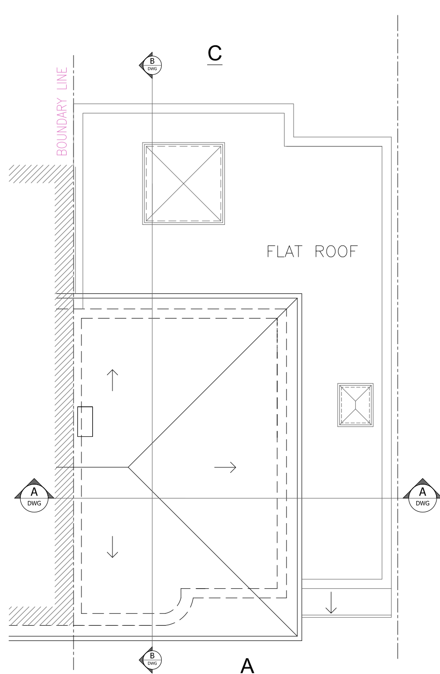
ROOF PLAN
