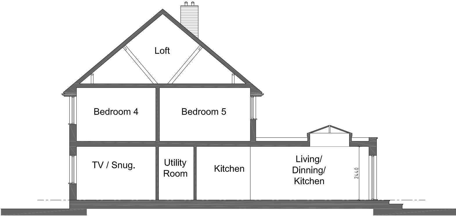
SECTION B-B
