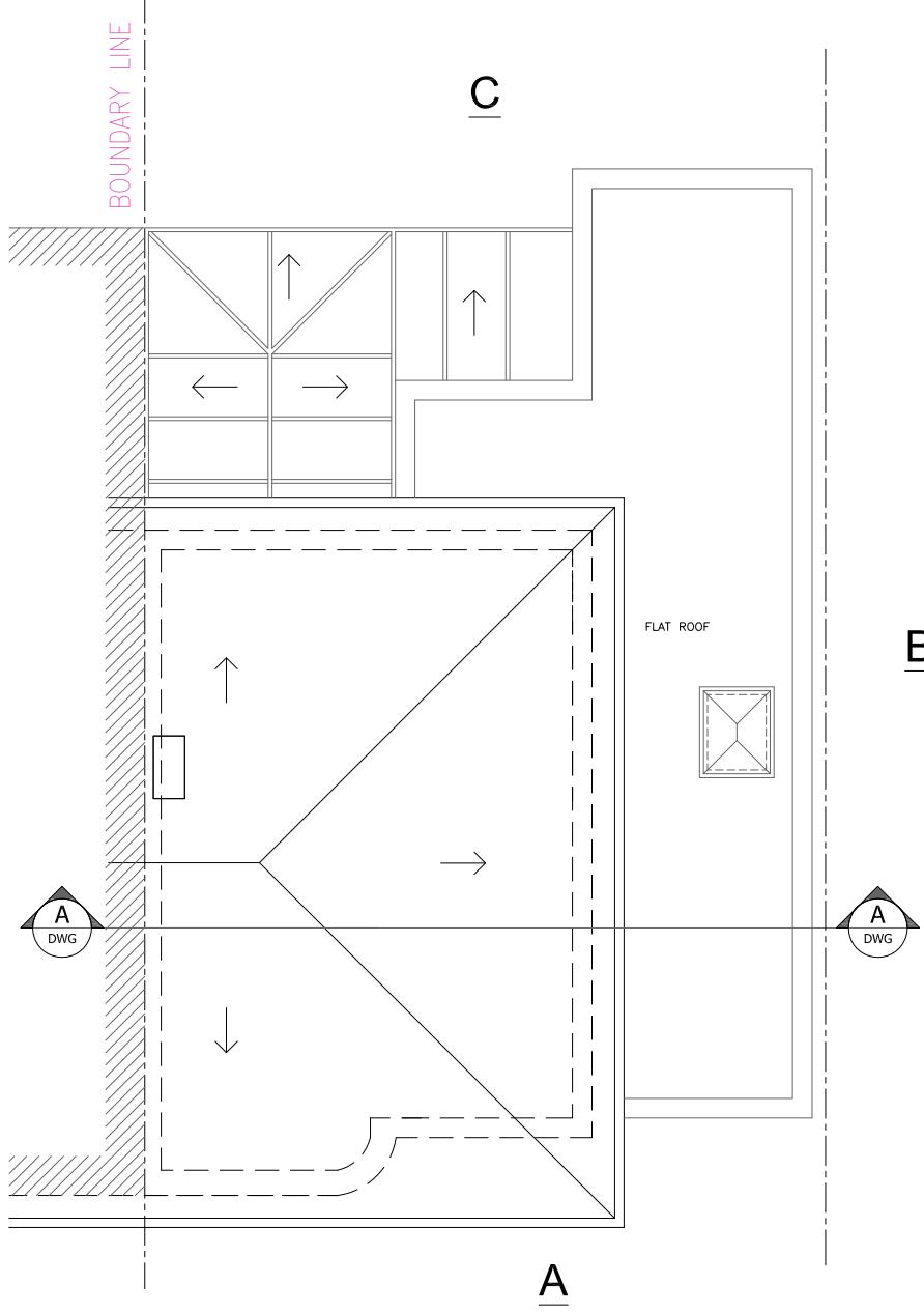
ROOF PLAN
